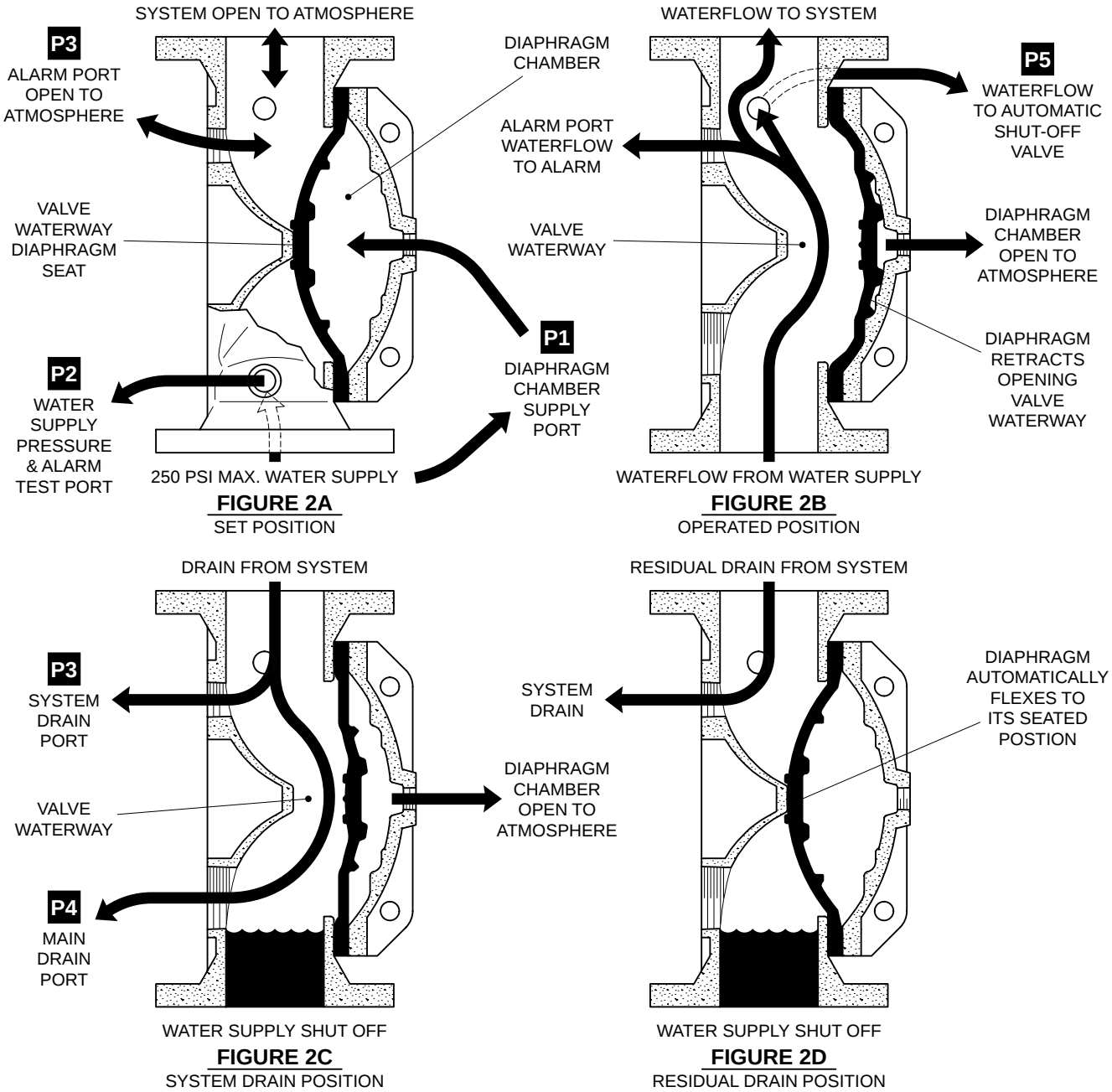
FIGURE 2 1-1/2 thru 8 INCH (DN40 thru DN200) MODEL DV-5 DELUGE VALVE — SET AND OPEN POSITIONS —
